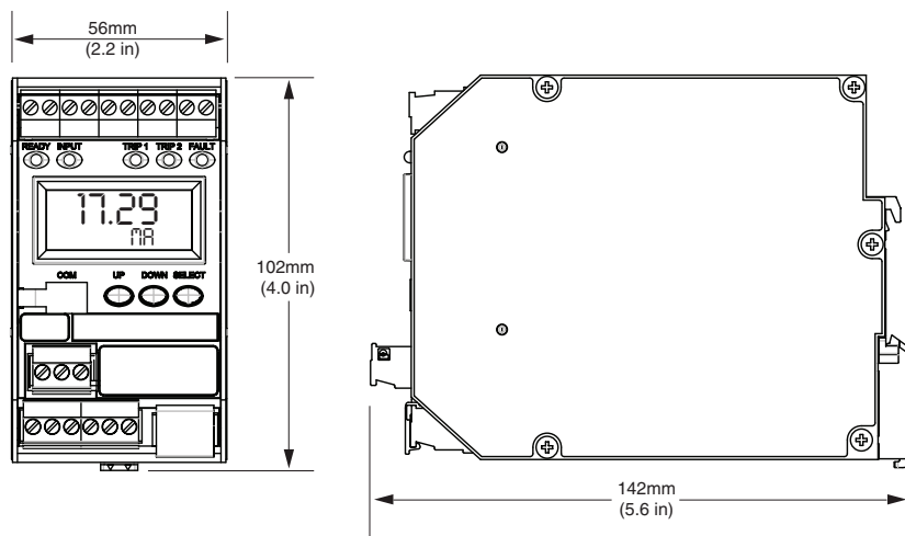
Figure 9. Installation Dimens:
